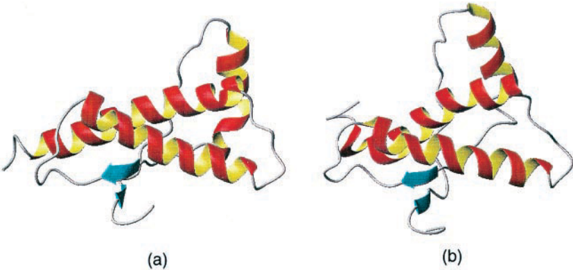
FIGURE 2 Molecular mechanics potential energy-minimized structures of the NMR-determined parts of HuPrP (a) and MoPrP (b).
