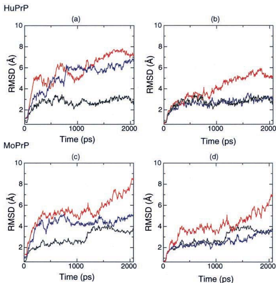
FIGURE 4 Root-mean-square deviations of the main chain atoms ((a) RMSD of the whole part of HuPrP, (b) RMSD of the globular domain of HuPrP, (c) RMSD of the whole part of MoPrP, and (d) RMSD of the globular domain of MoPrP). Black, blue, and red lines indicate RMSDs of the control, wild, and mutant structures, respectively. With regard to the initial states of MD simulations, the structures of these globular domains were very similar. The ordinate is RMSD (Å), and the abscissa is time (ps).
